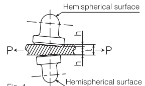
Fig. 1 Depth to which the teeth cut into the load : h
