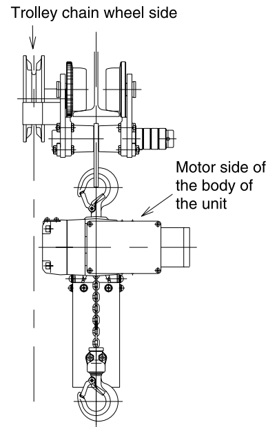
Fig. 8 For a geared trolley of 125 kg to 200 kg
