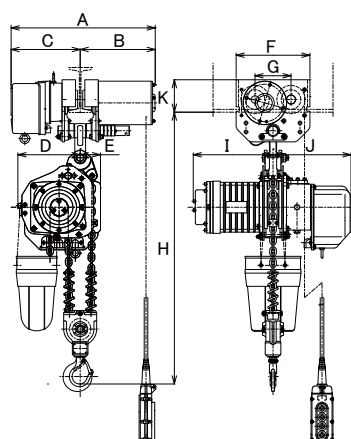
1w ~ 5ton The drawing of electric trolley 3t, 5t is different from above drawing.
